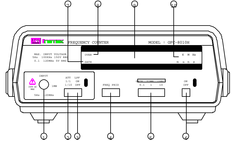
Fig. 1 Front panel
