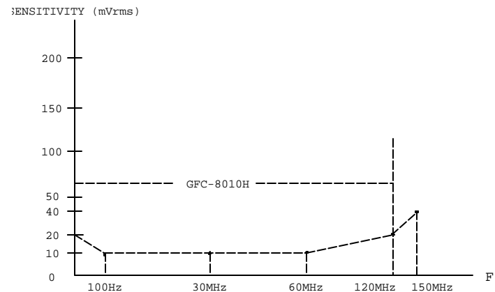
Fig. 5 Input Sensitivity Characteristic
