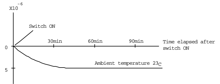
Fig. 9 Example of crystal oscillator rise characteristics
